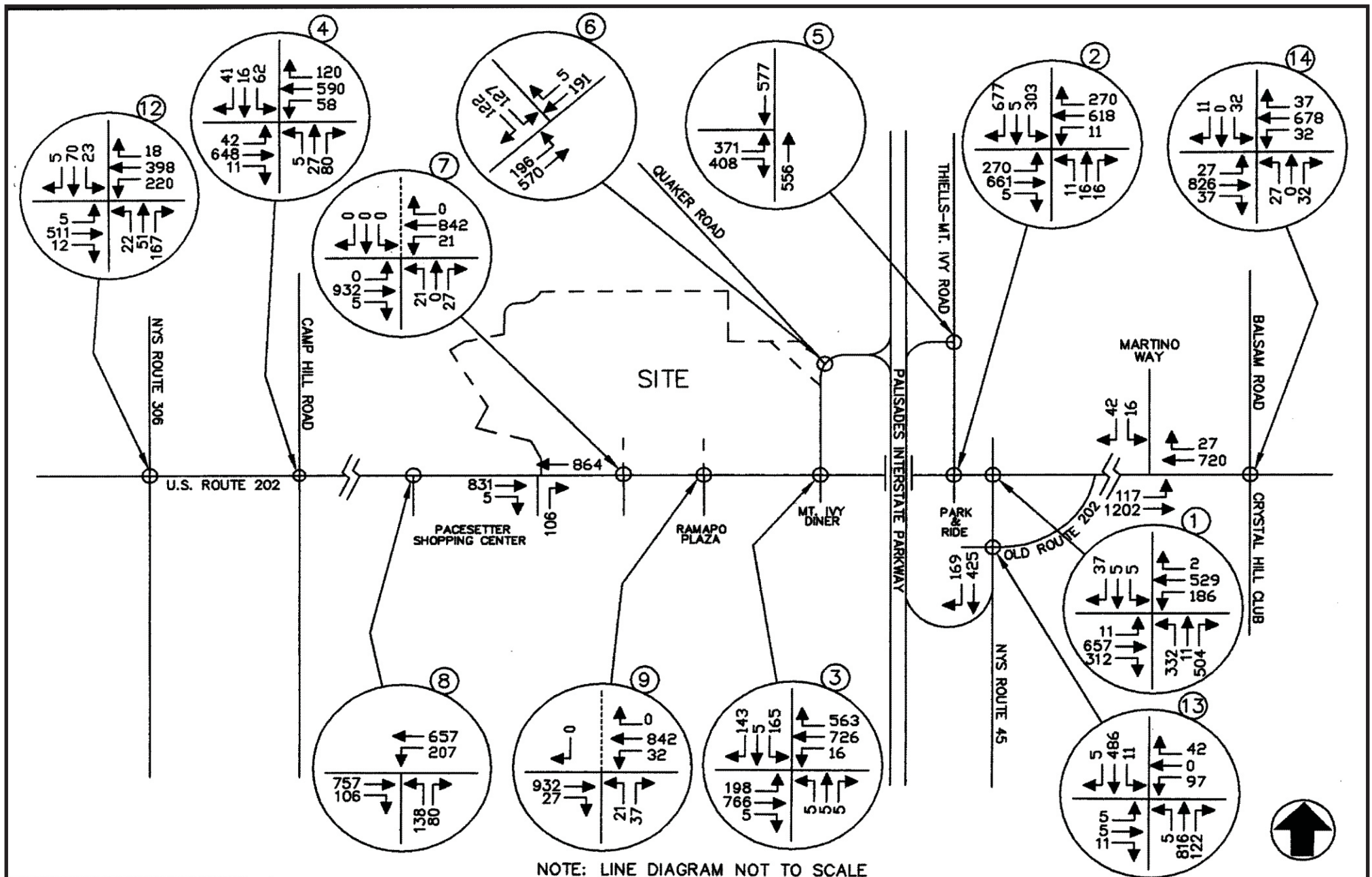
Figure 3.5-31: 2011 No-Build Traffic Volumes Weekday Peak PM Highway Hour (With Patrick Farm) Minisceongo Park Towns of Haverstraw & Ramapo, Rockland County, New York Source: John Collins Engineers, P.C. Date: October, 2008
